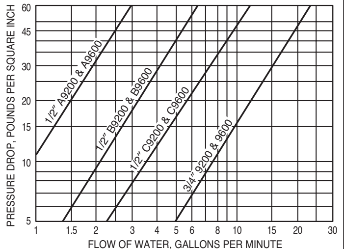
FLOW CAPACITIES - SERIES 9200 & 9600
