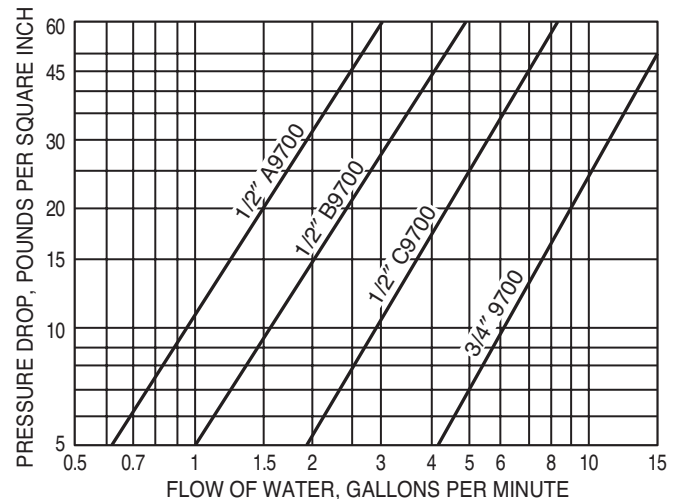
FLOW CAPACITIES - SERIES 9700
