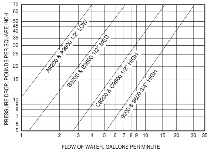
FLOW CAPACITIES SINGLE STAGE - SERIES 9200 & 9600
